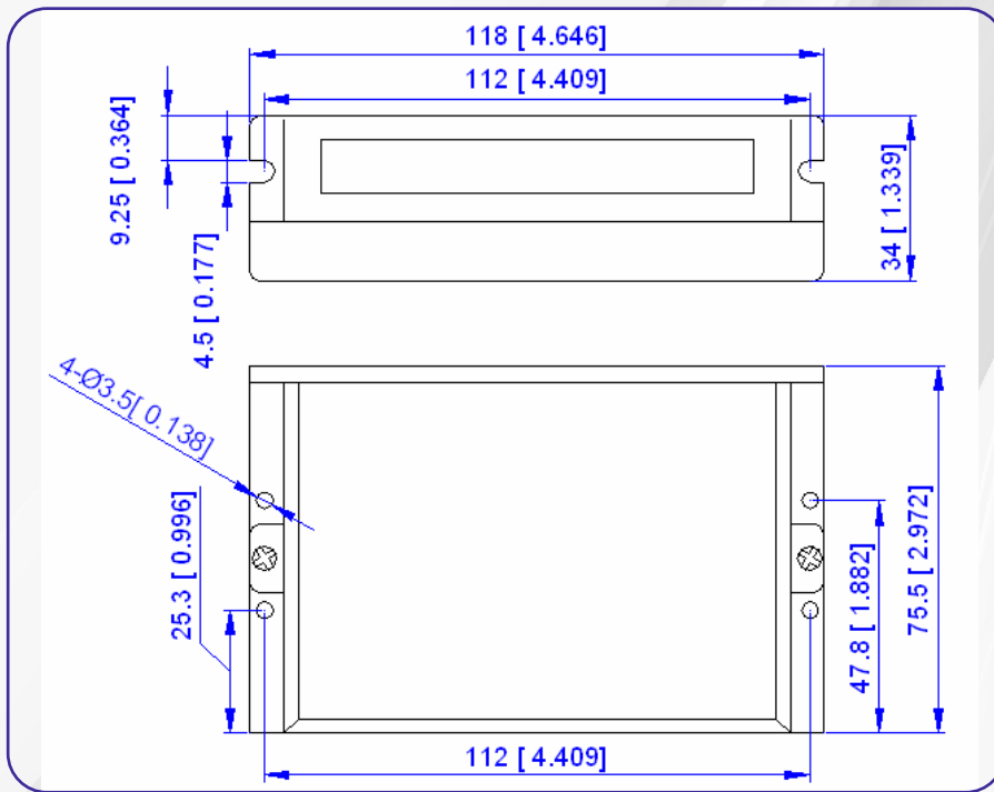
Figure 1: Mechanical specifications
